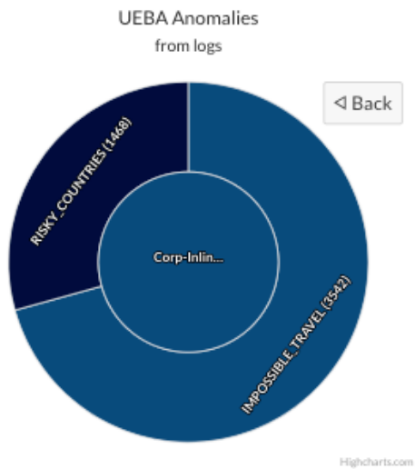
Anomaly Counts
